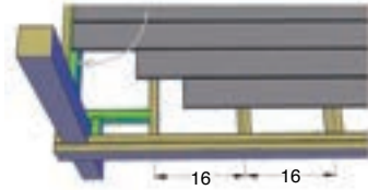
Additional cleat to support Zuri trim
